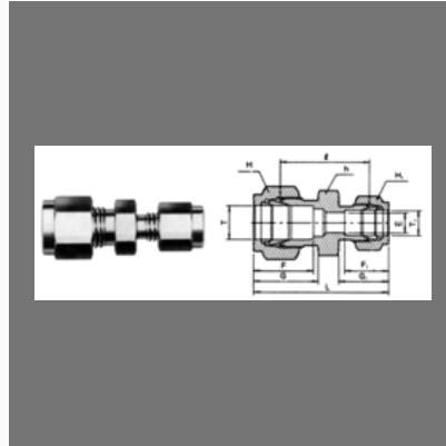
Reducing Union
