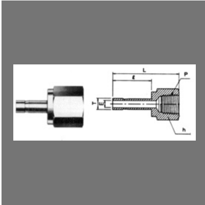
Female Adapter
